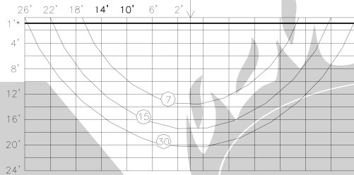
3/8" ORIFICE-K=2.8
