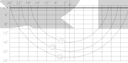
17/32" ORIFICE-K=8.1
