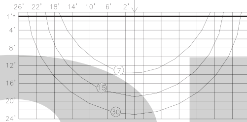
7/16" ORIFICE-K=4.2
