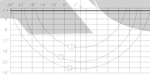
1/2" ORIFICE-K=5.6
