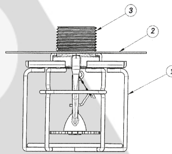
1 - Guard, Model 25 2 - Shield, ESFR 3 - Sprinkler Assy, Model N25 ESFR
