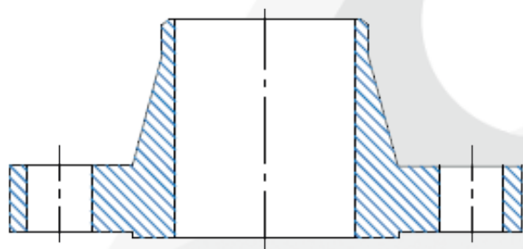
BRIDA WELDING - NECK
