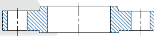
BRIDA SLIP-ON
