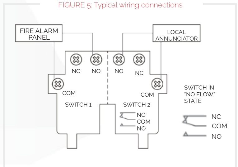
FIGURE 5: Typical wiring connections
